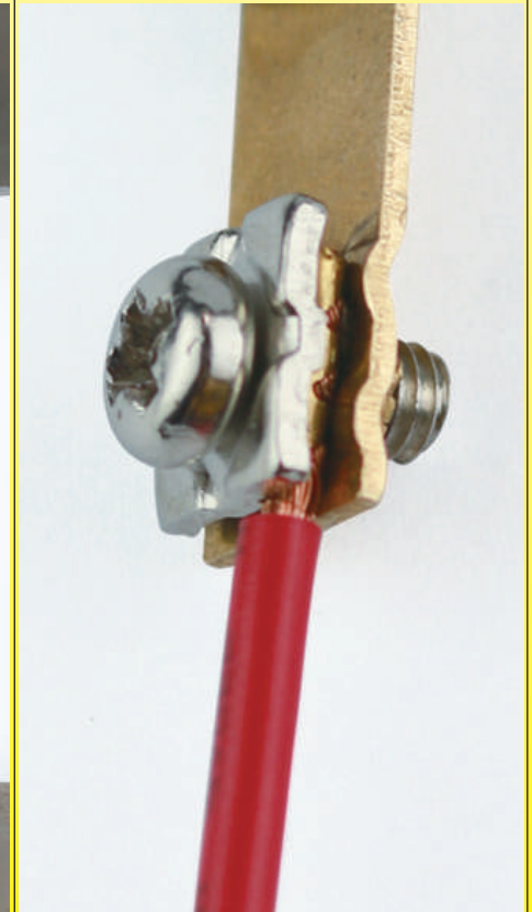
Terminal detail
